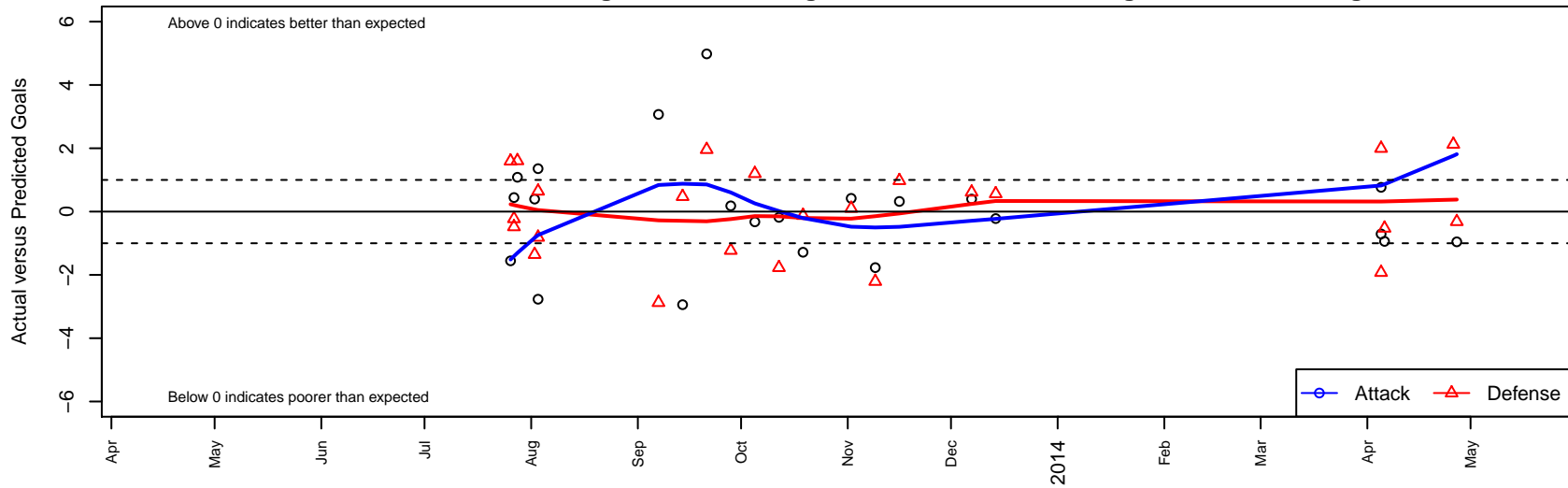
NK Fire B02 Dots are actual minus expected GF (blue circles) and GA (red triangles). Blue line is smoothed change in attack strength. Red is smoothed change in defense strength.
